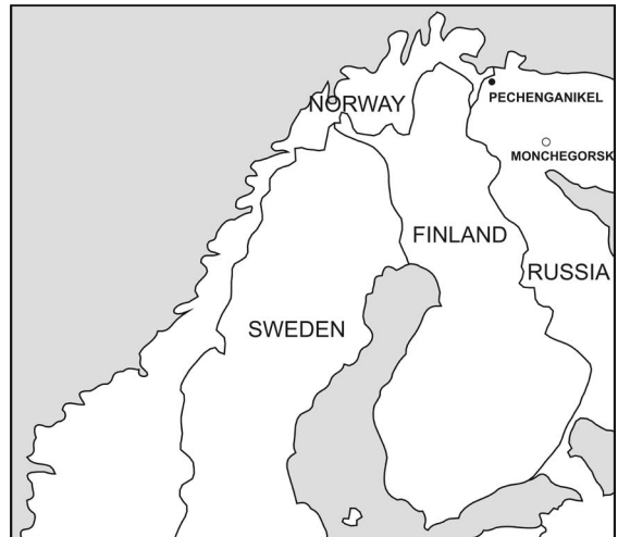
Figure 1: Pechenganikel (the study area) and Monchegorsk smelters in Kola Peninsula.
