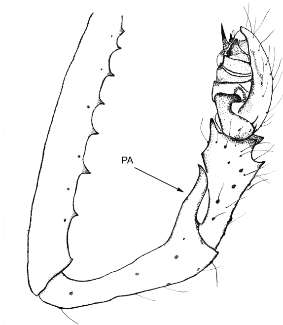
Fig. 3: Prinerigone vagans (Audouin, 1826) from Poland, left male pedipalp, retrolateral view (Scale line = 0.2 mm; PA = patellar apophysis)
