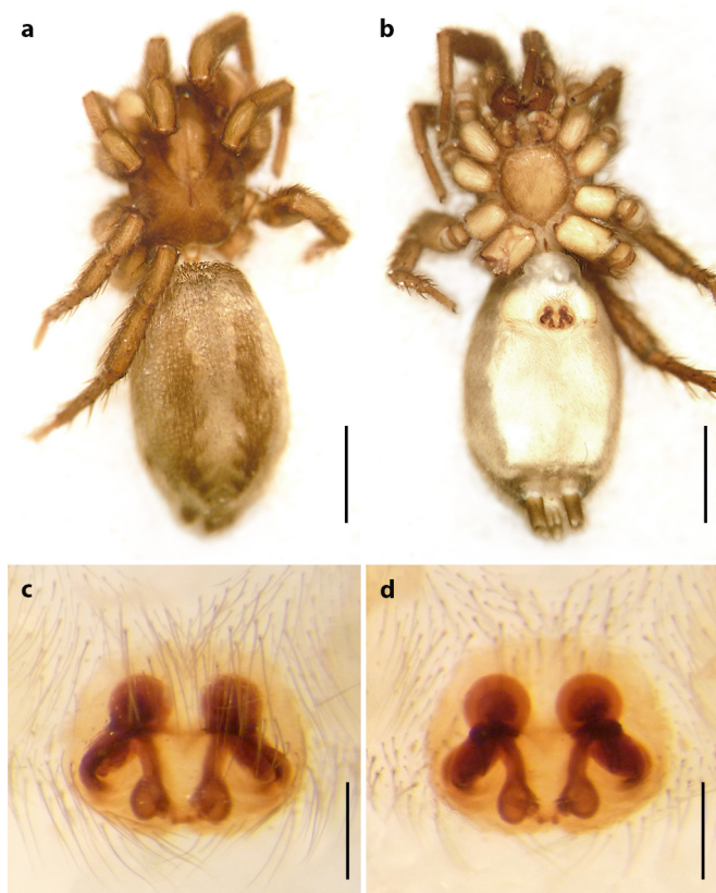
Fig. 17: Nomisio peloponnesiaca , female. a. dorsal; b. ventral view; scale lines: 1.7 mm; c. epigyne, ventral views; d. vulva, dorsal views; scale lines: 0.27 mm
